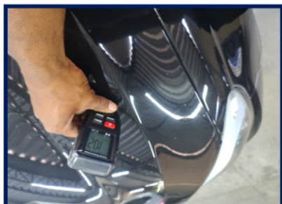
PARACHOQUE DIANT
